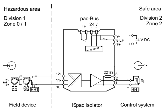
Connection diagram 9160/13-11-11
