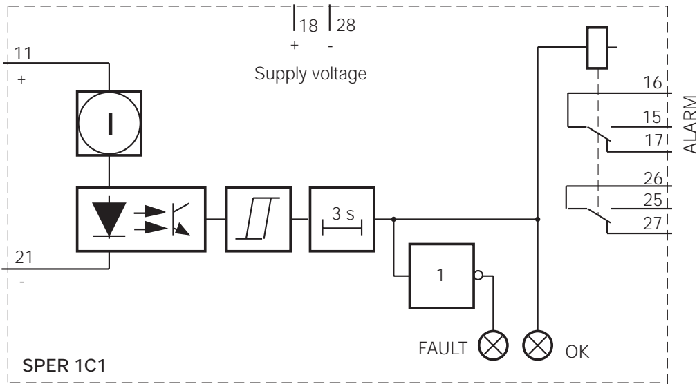
Fig. 1 Block diagram
